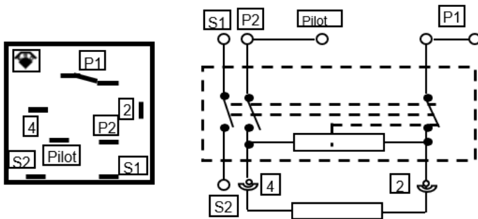
Wiring diagram in 'O' position:
