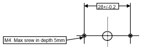
Mounting Dimensions:
