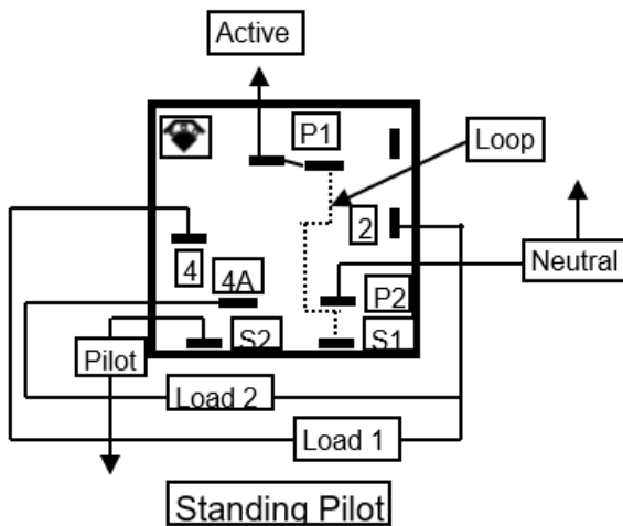
Wiring diagram in 'O' position:
