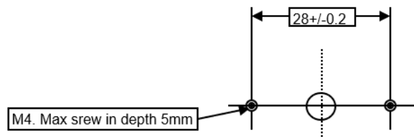
Mounting Dimensions:
