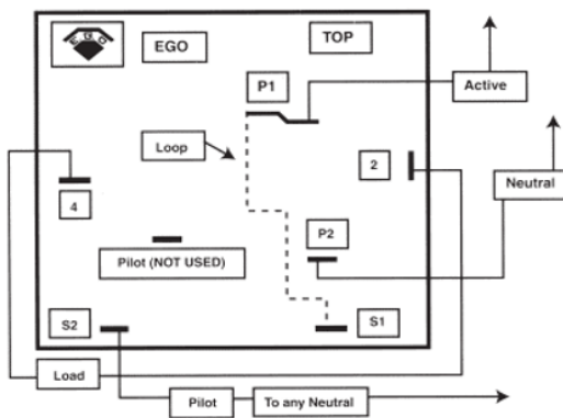
Wiring diagram in 'O' position:
