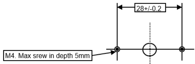
Mounting Dimensions:
