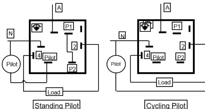
Wiring diagram in 'O' position:
