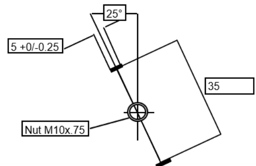
Mounting Dimensions:
